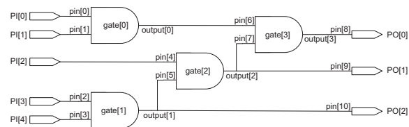
(a) A sample circuit
